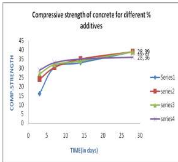
Graph 2 : For M35 Concrete
